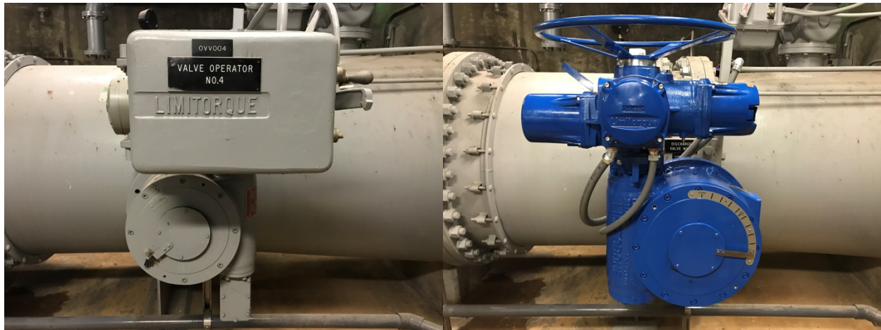
Old Gear Drive & Actuator
